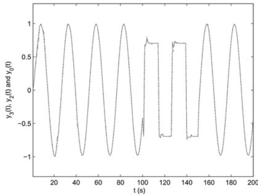
Fig. 8 Control results. Method 2: IENN SOQARX-RBFN control output using optimized M = 4 (solid), IENN QARX-RBFN control output using fixed M = 6 (dashed) and reference (dotted).
