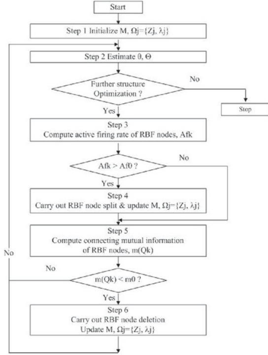
Fig. 1 Flowchart of self-organization of the ARX-RBFN model.
