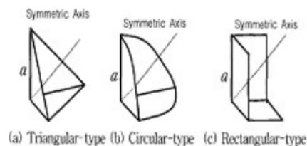
Figure 3. Radar Reflector Type (Yim and Kim, 2003)
