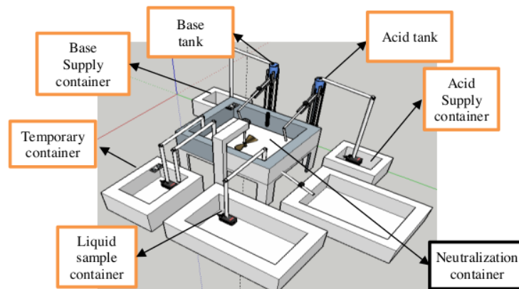
Figure 1 Design of pH neutralization process
