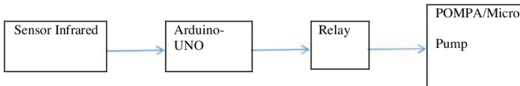
Gambar 1. Blok Diagram
