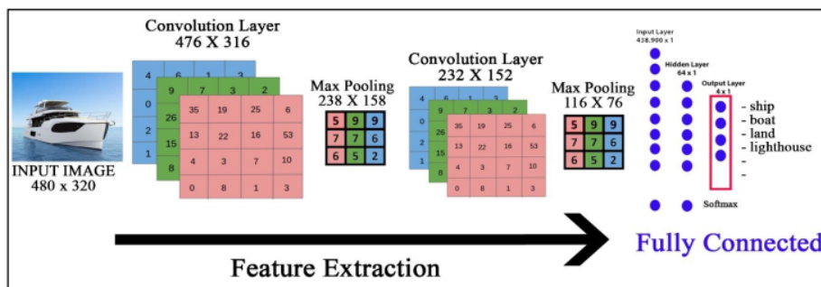
Figure 2. CNN architecture.
