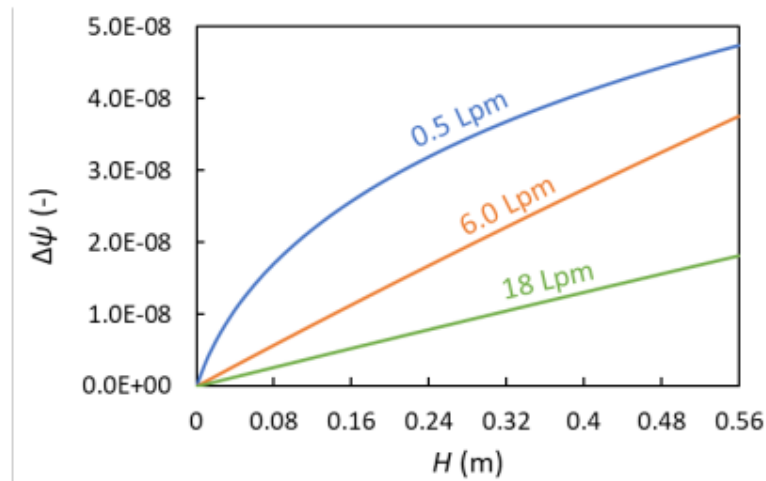
Figure 9: Increased relative humidity along the tower height.
