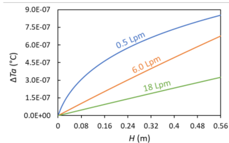
Figure 8: Increased air temperature along the tower height.
