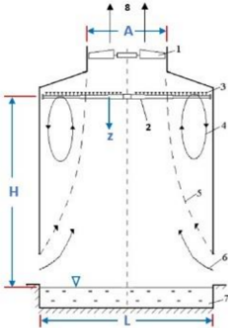
1 Figure 1: Scheme of the cooling tower: (1) Exhaust fan, (2) Delivery pipe, (3) Spraying nozzles, (4) Stagnation zone, (5) Line of stagnation zone, (6) Enter air, (7) Water basin, (8) Exit air.
