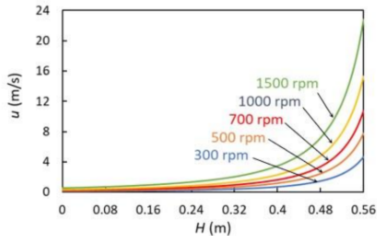
Figure 10: Air velocity along with tower height.
