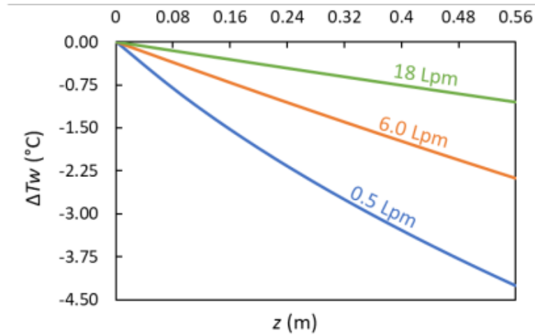
Figure 7: Decreased droplet temperature along its trajectory.
