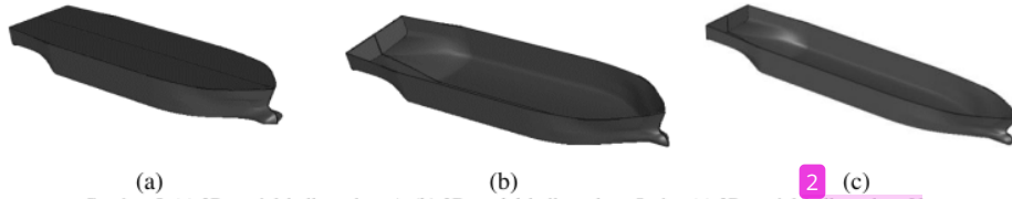
Gambar 5. (a) 3D model bulbous bow Δ, (b) 3D model bulbous bow Ω, dan (c) 3D model bulbous bow V
