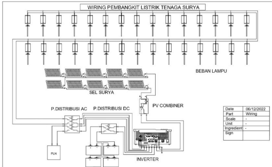
Figure 1. Floating PLTS System and Wiring
