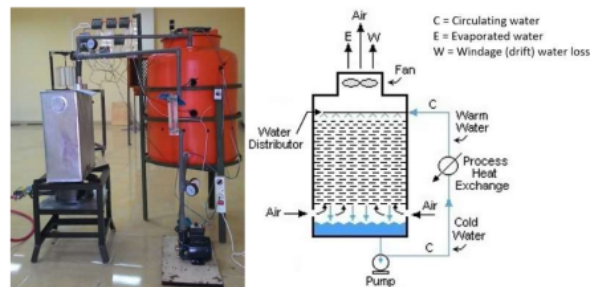
Figure 1 Experimental setup and apparatus.
